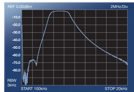
Band Pass Filter (7MHz, Span 20MHz)
