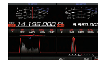
Expanded Filter Function Display
