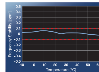
±0.1 ppm High Precision TCXO
